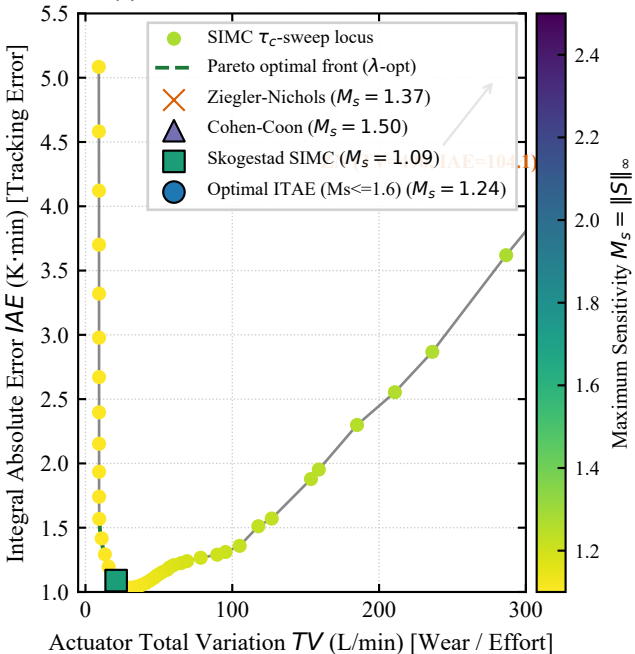
(a) True Pareto Trade-off: IAE vs TV
