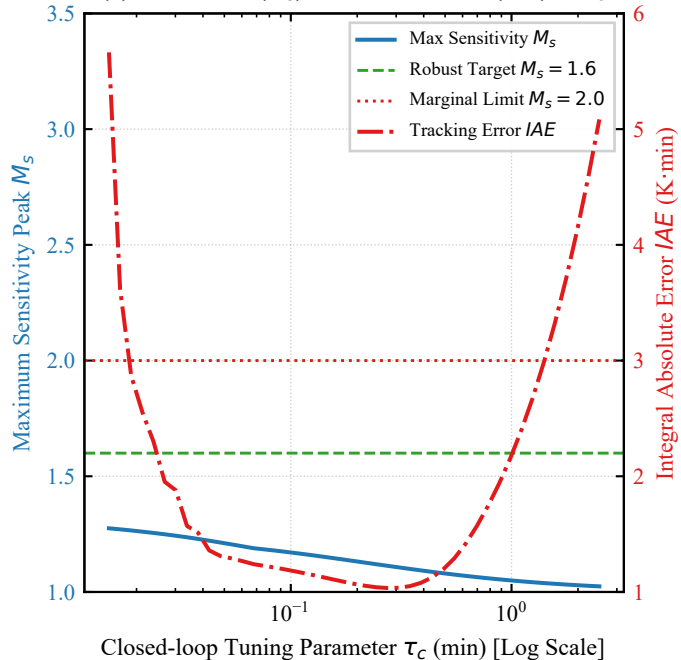
(b) Robustness ( M_s ) and Performance ( IAE ) vs \tau_c
