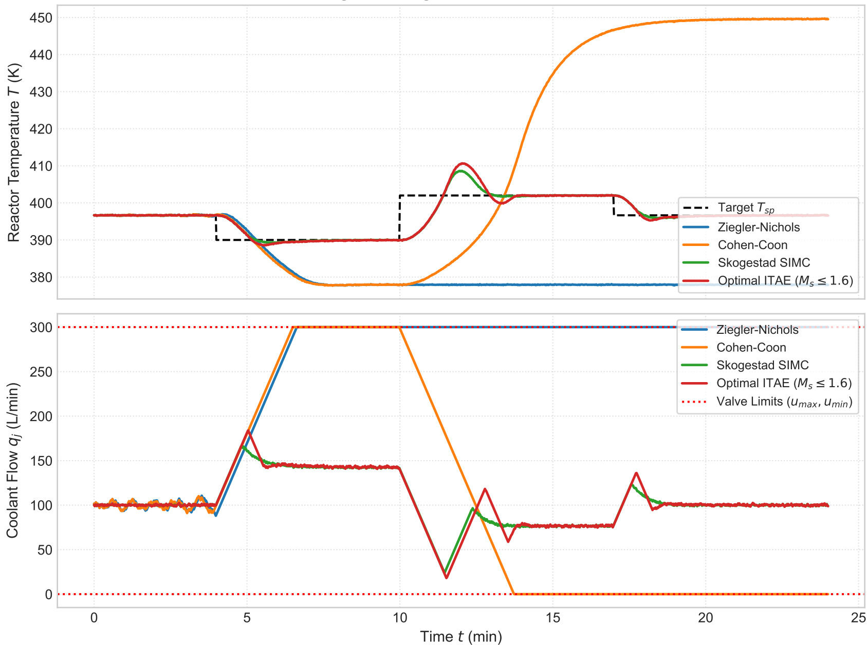
Non-linear Wide-Range Tracking: 396.65 K \rightarrow 390 K \rightarrow 402 K \rightarrow 396.65 K
