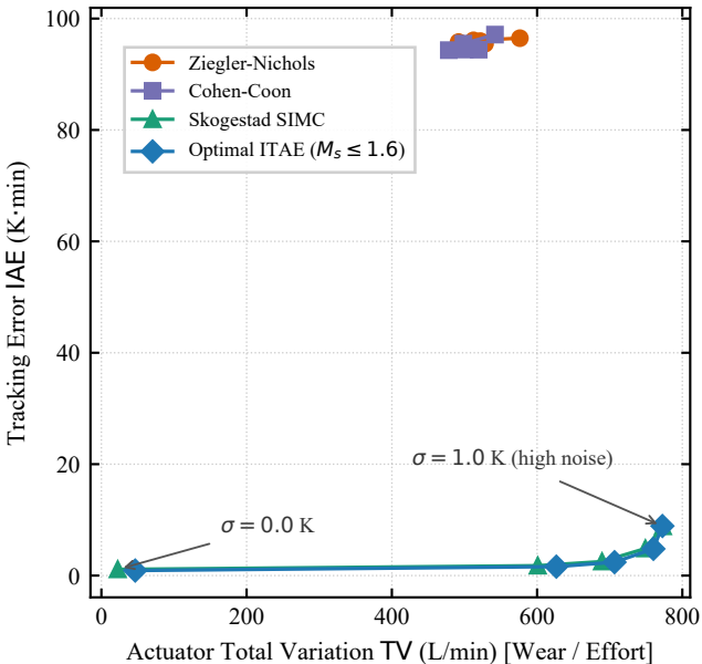
Noise Sensitivity: Tracking Quality vs Actuator Wear
