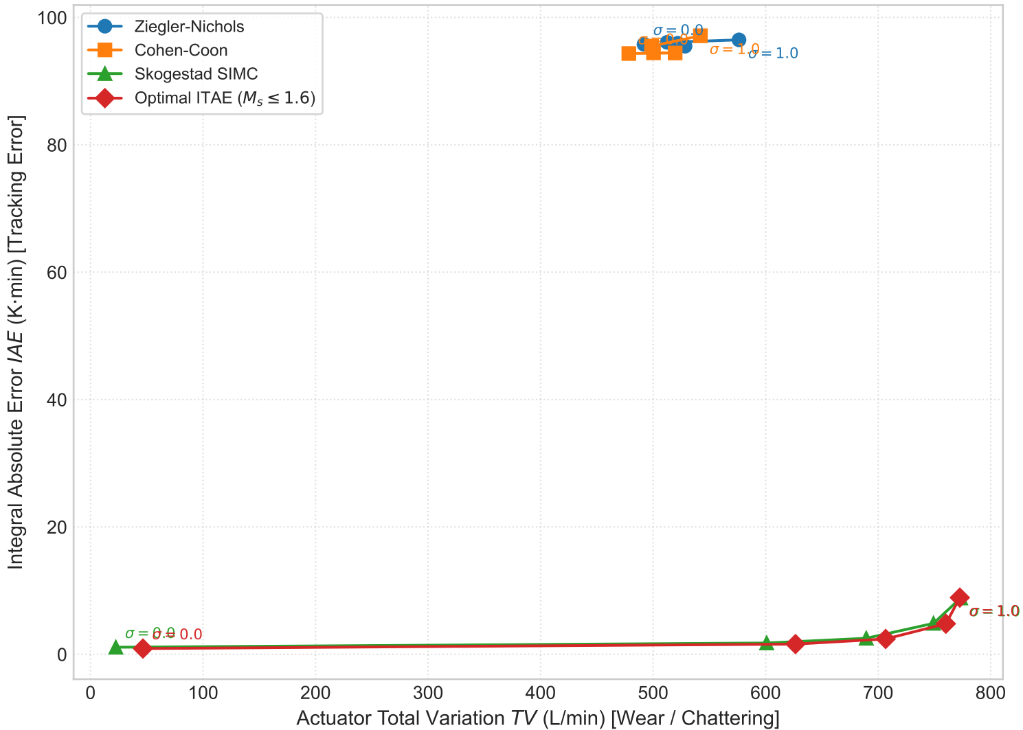
Pareto Trade-off: Tracking Quality vs Actuator Wear across Noise Levels
