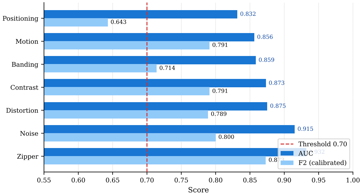
Per-Class Performance (v7, calibrated thresholds)
