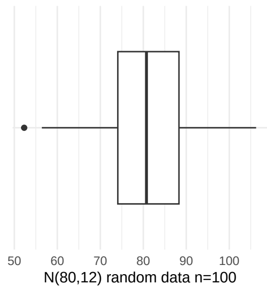
Figure 3.16: Simulated normal data, n=100 and n=1000
