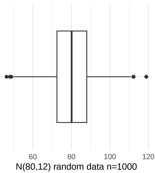
Figure 3.16: Simulated normal data, n=100 and n=1000
