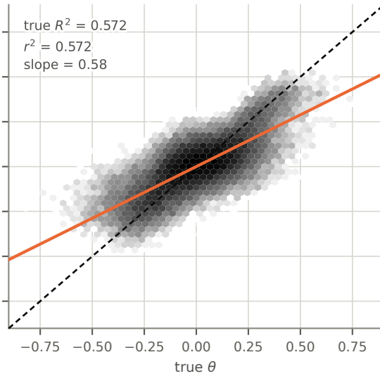
CloneAtt-NPE
