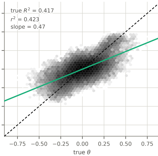
CloneMLP-NPE
