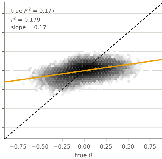
DominantClone-NPE
