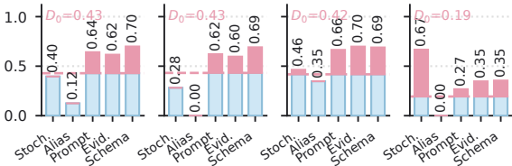
Mean drift
