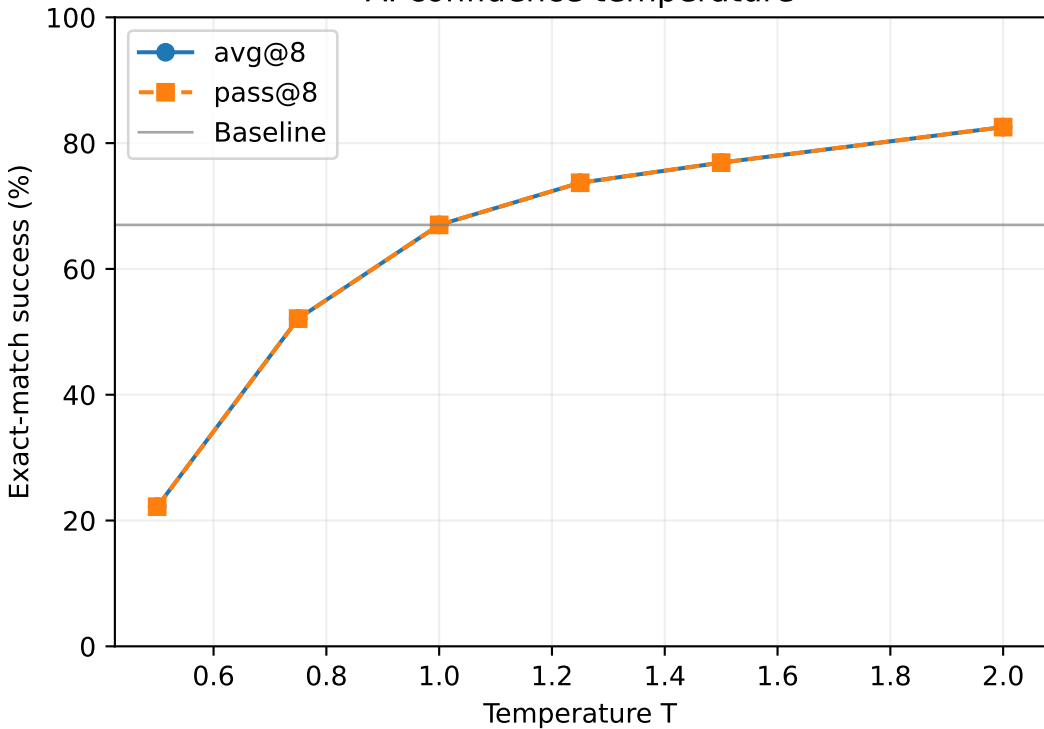
A: confidence temperature
