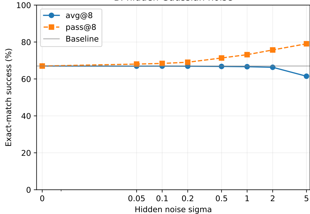
B: hidden Gaussian noise
