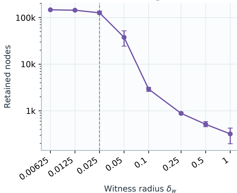
Pruning
