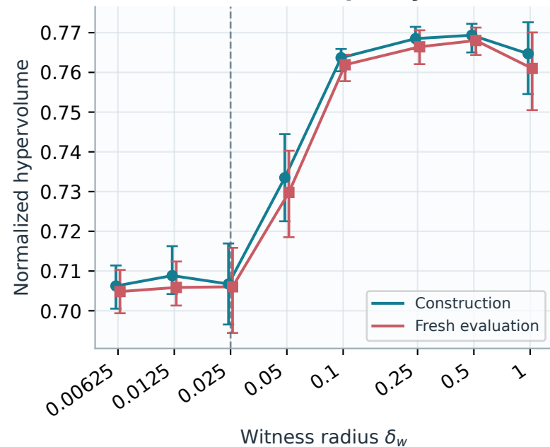
Solution quality
