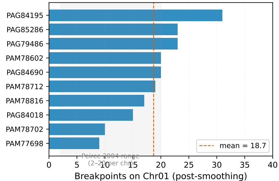
A. Per-line recombination density
