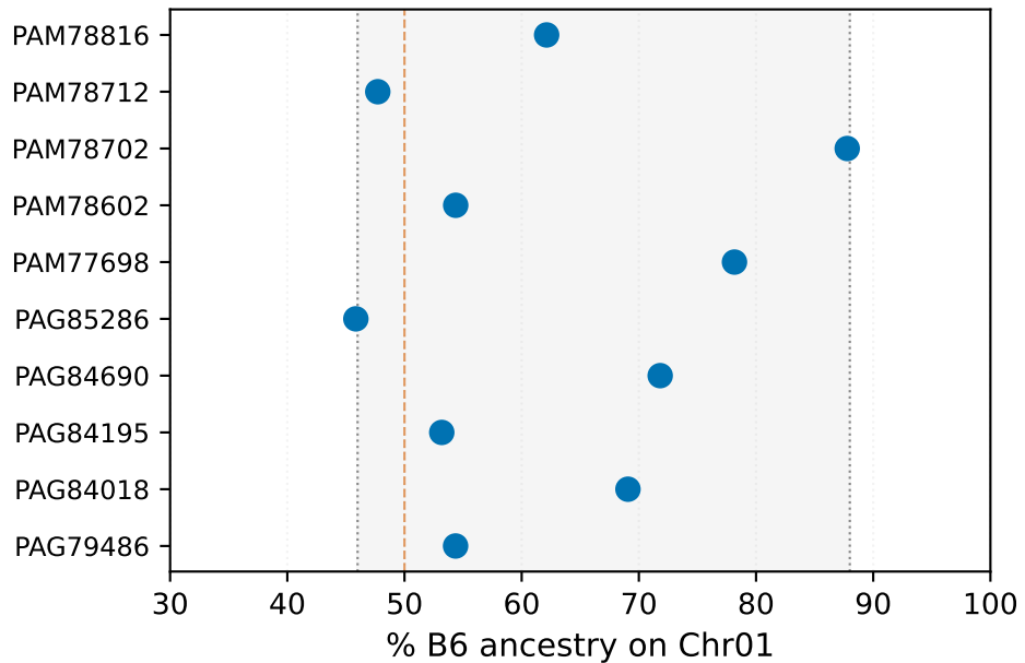
B. B6 ancestry fraction per line (paper: 46-88%)
