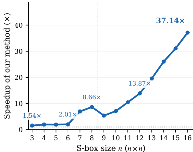
(b) Speedup ↑
