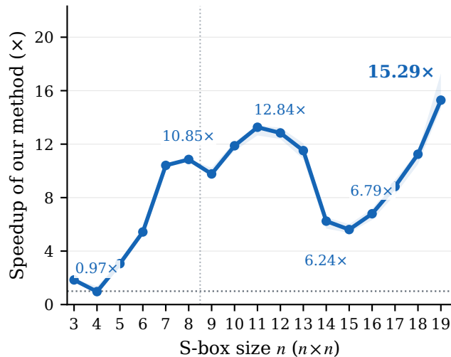
(b) Speedup \uparrow
