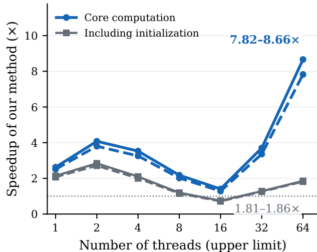
(b) Speedup at equal thread counts ↑
