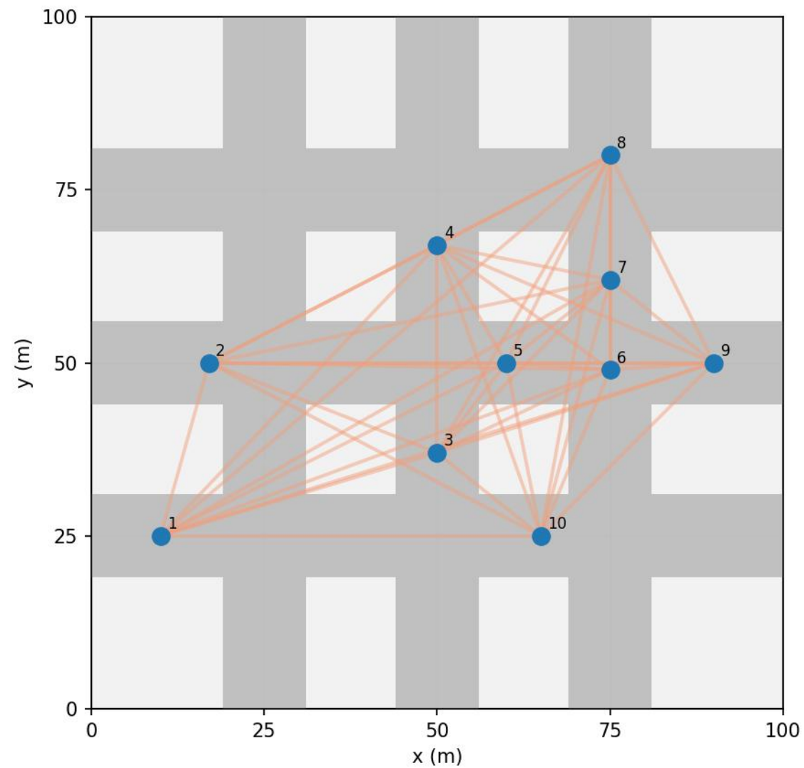
B. Mesh Topology
