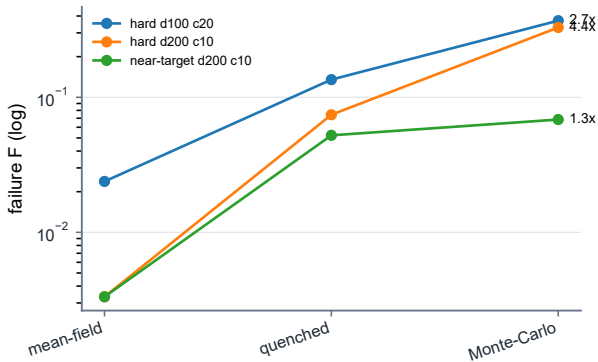
Failure rises with evaluator fidelity
