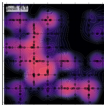
Communication delay
