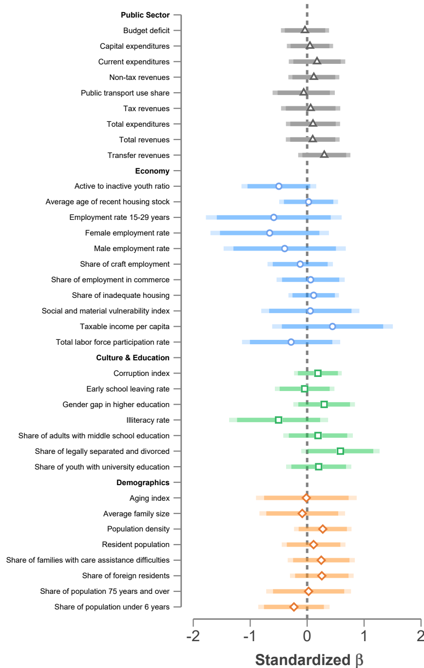
Figure 6: Balance Tests
