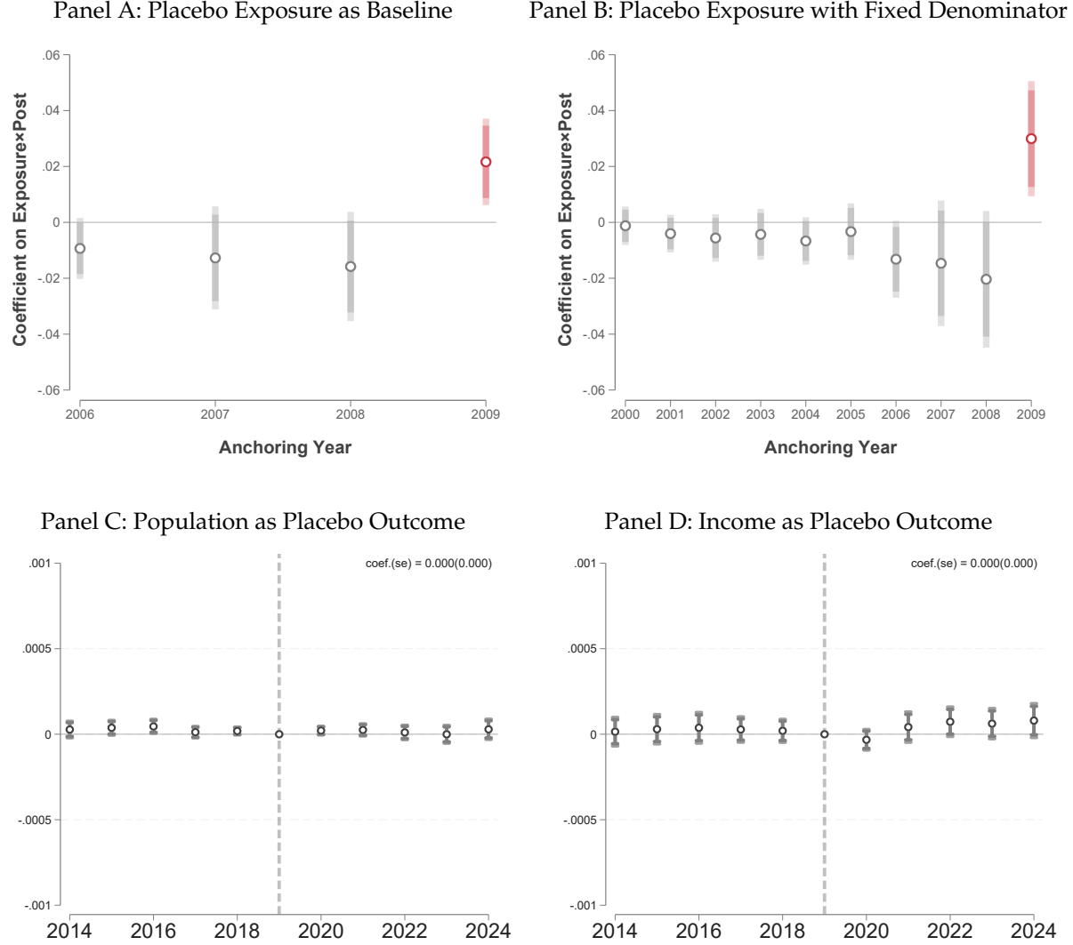
Figure 7: Falsification Tests
