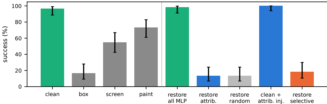
Closed loop: 5 tasks x 12 paired episodes; restores under 'box'
