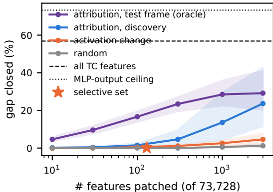
pi0.5 / LIBERO-Spatial [box (rendered)]
