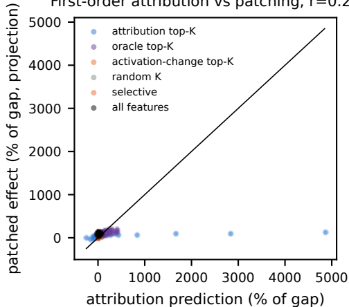
First-order attribution vs patching, r=0.28
