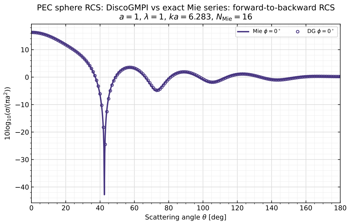
Figure 10.7: Forward-to-backward RCS cut for the MN5 EPW4/P4 run. Here \theta = 0^\circ is the forward +z direction and \theta = 180^\circ is the backscatter direction.
