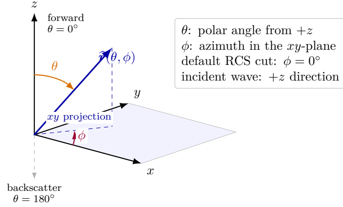
Figure 10.1: DiscoGMPI angular convention for RCS observation directions. The polar angle \theta is measured from the +z axis, while the azimuth \phi is measured in the xy -plane from +x toward +y .
