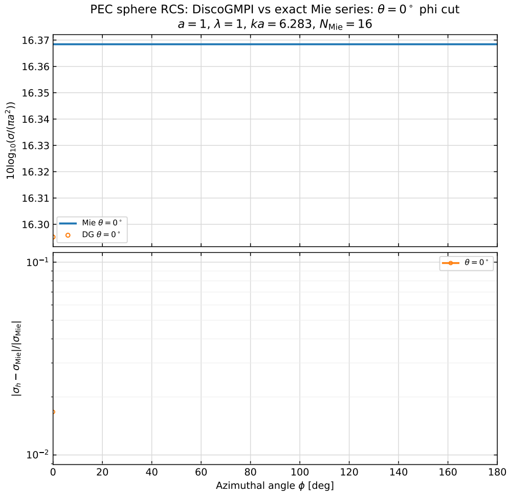
Figure 10.9: \theta = 0^\circ azimuthal diagnostic produced by the MN5 EPW4/P4 postprocessor. This run requested only \phi = 0^\circ , so the DG data contain one azimuth sample. The figure is therefore a bookkeeping and orientation check, not a full \phi -sweep validation.
