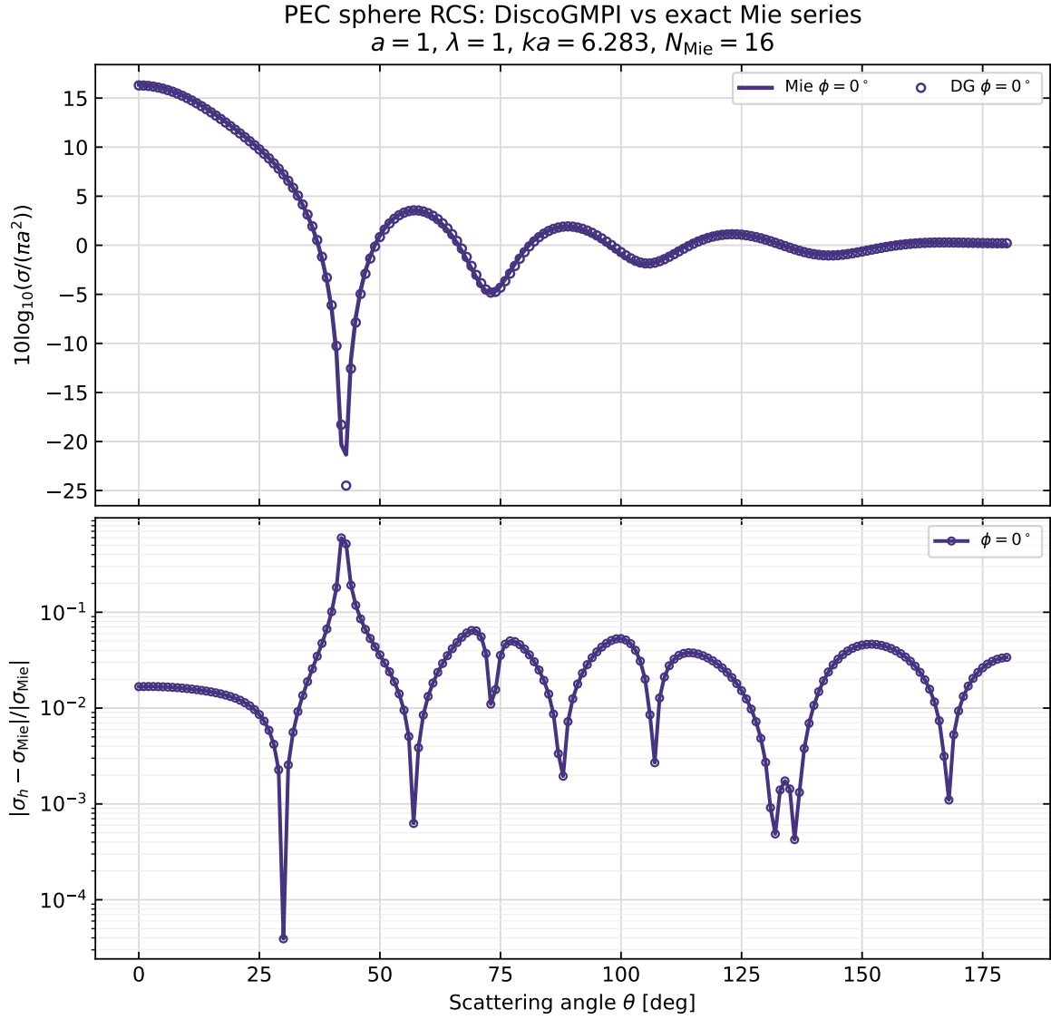
Figure 10.6: MN5 EPW4/P4 Cartesian RCS comparison. The upper panel compares the DG near-to-far result with the exact Mie curve for 10 \log_{10}(\sigma/(\pi a^2)) . The lower panel reports the relative error; the visible peaks correspond mainly to angular neighborhoods of Mie nulls.
