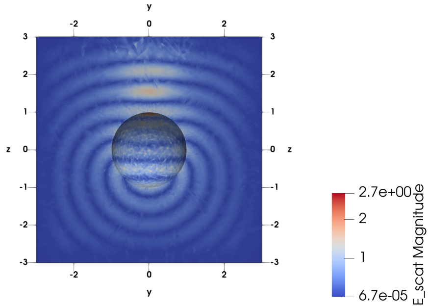
Figure 10.5: Scattered-field visualization from the MN5 EPW4/P4 run. The outgoing pattern around the sphere is the field used by the near-to-far RCS extraction after the time-windowed Fourier transform.
