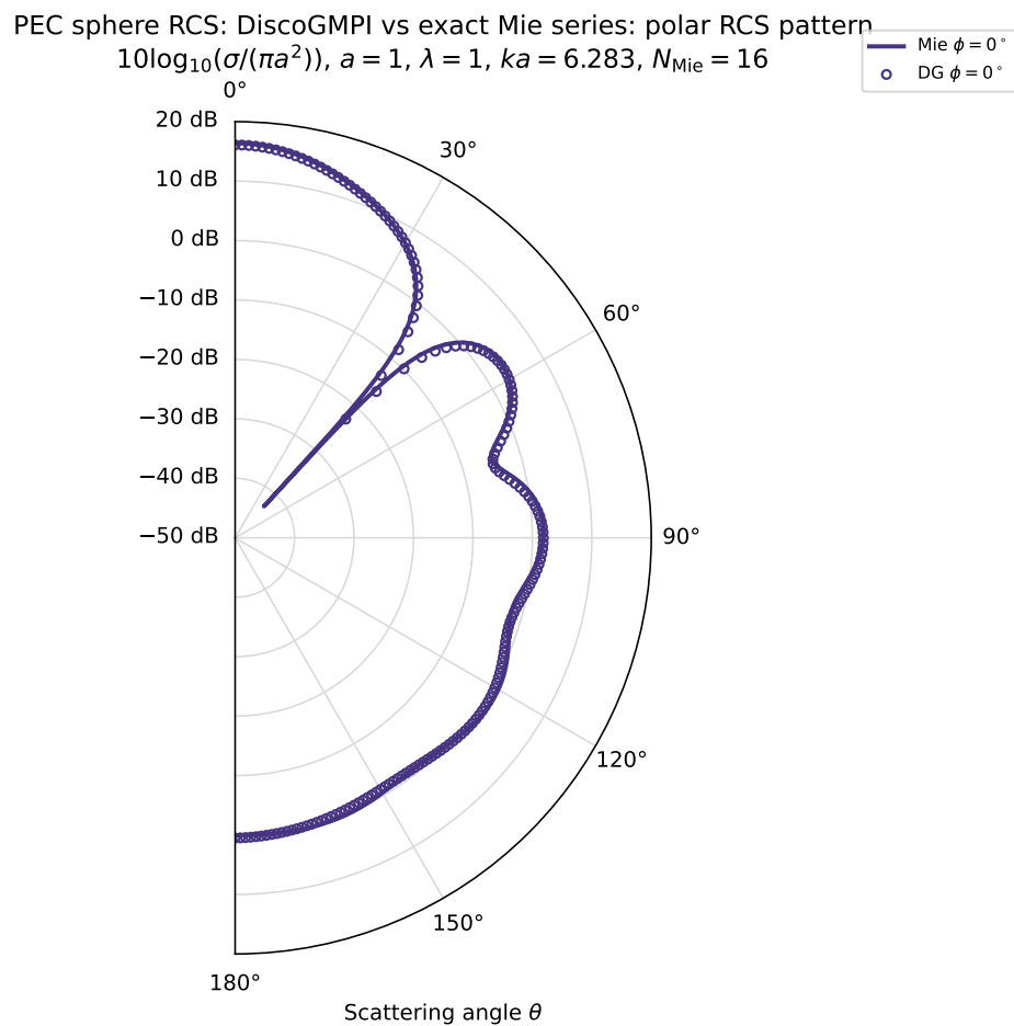
Figure 10.3: Polar RCS pattern for the same run. The angular coordinate is the DiscoGMPI polar scattering angle \theta , with \theta = 0^\circ denoting the forward +z direction and \theta = 180^\circ denoting backscatter. The radial tick labels are normalized dB values, 10\log_{10}(\sigma/(\pi a^2)) .
