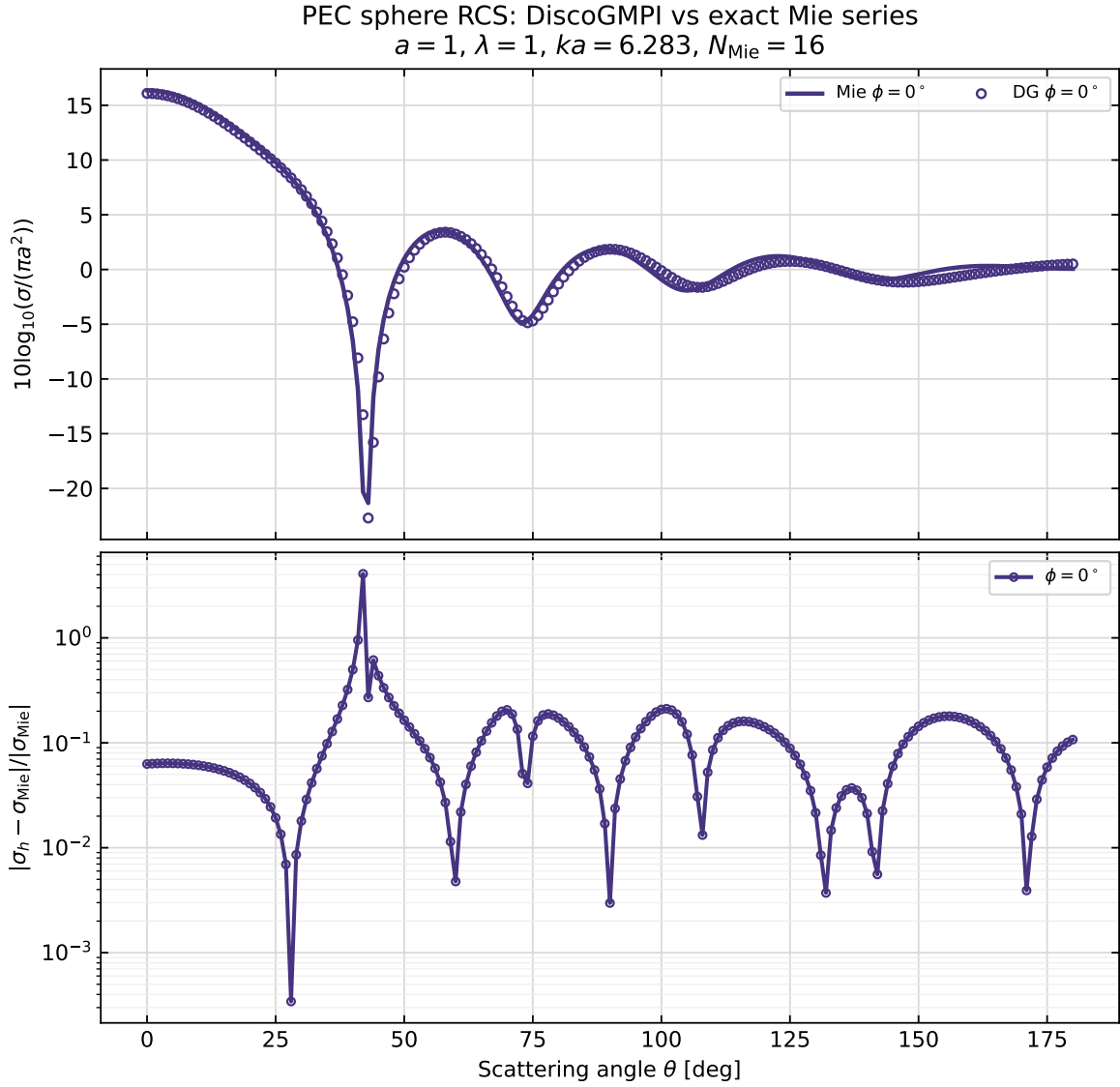
Figure 10.2: Cartesian RCS comparison for the coarse_sphere_rcs_epw2_p4_transient_theta181 run. The upper panel compares 10 \log_{10}(\sigma/(\pi a^2)) for the DG near-to-far extraction and the exact PEC-sphere Mie series. The lower panel reports the relative RCS error.
