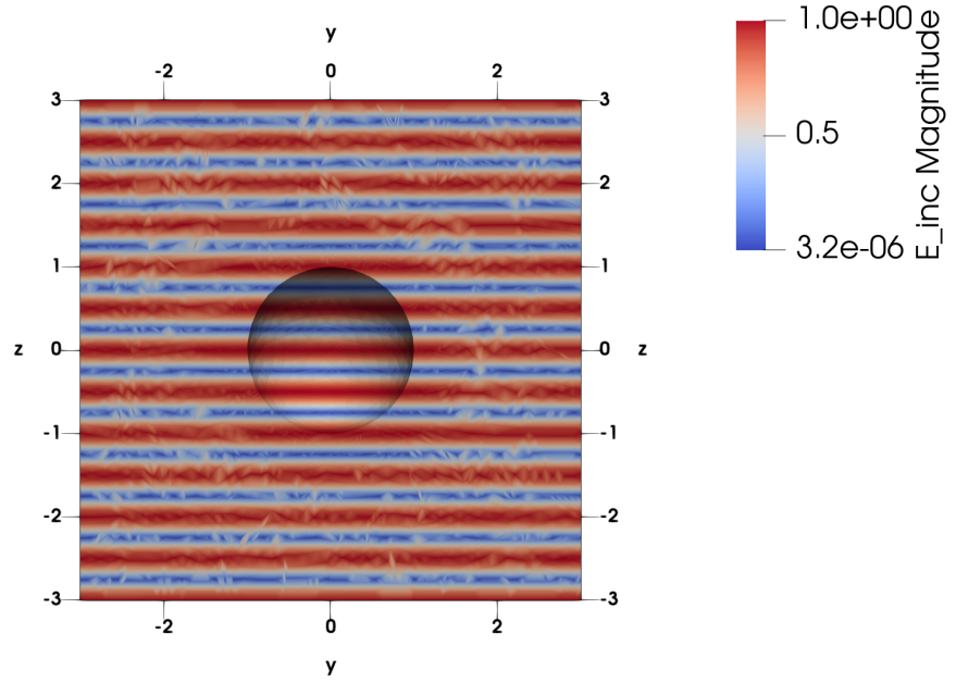
Figure 10.4: Incident-field visualization from the MN5 EPW4/P4 run. The plot shows the imposed +z -propagating, x -polarized plane wave used to construct the total field and the incident-aware PEC boundary condition.
