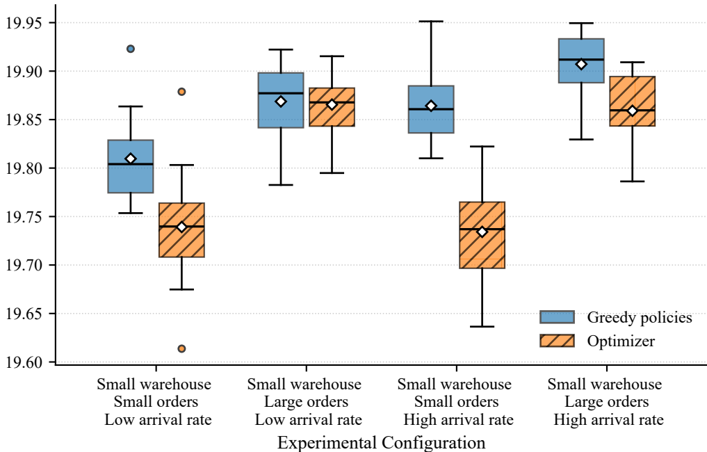
Average number of pods moving
