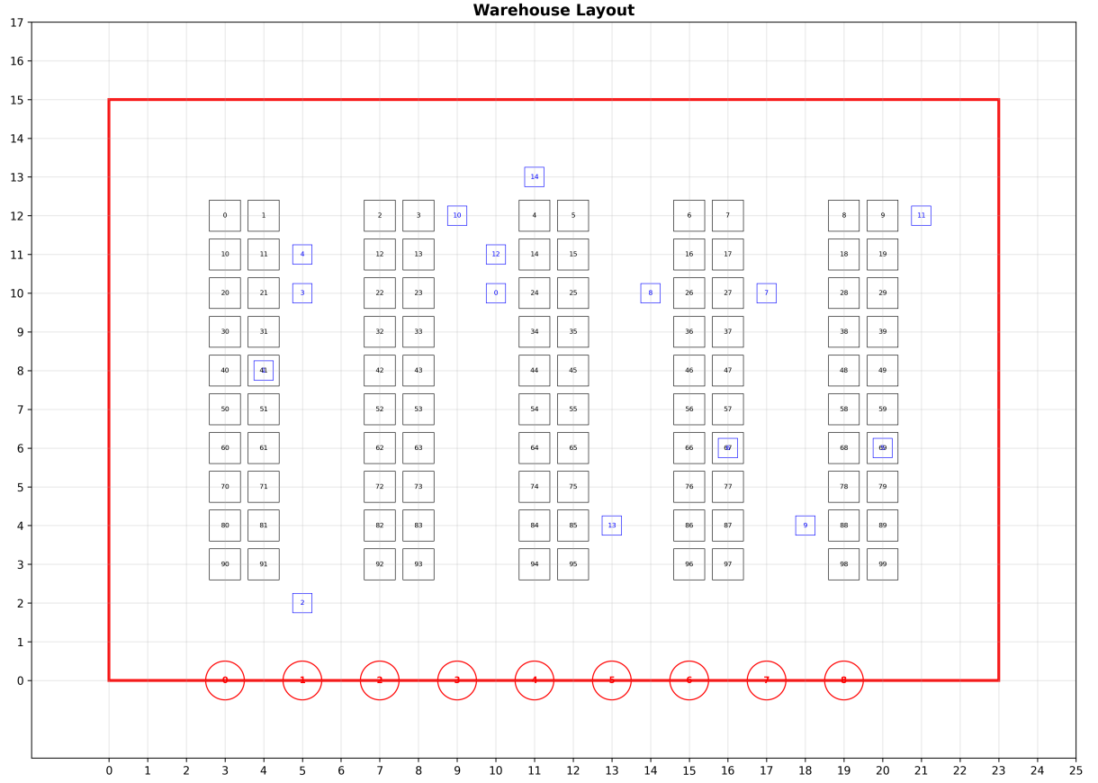
Figure 1: Example layout created with GRID_ROWS = 10 , GRID_COLS = 10 , NUM_ROBOTS = 15 and NUM_WORKSTATION = 9 .
