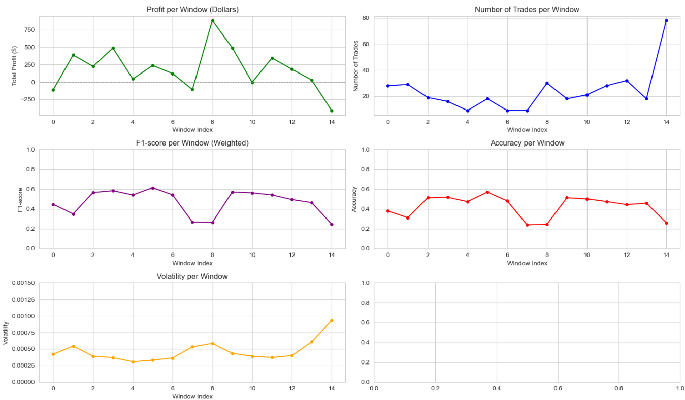
Rolling Window Backtest Performance Metrics
