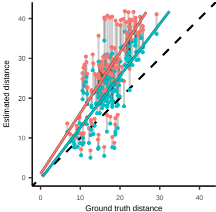
Estimated vs. True Distances, cta-seq
