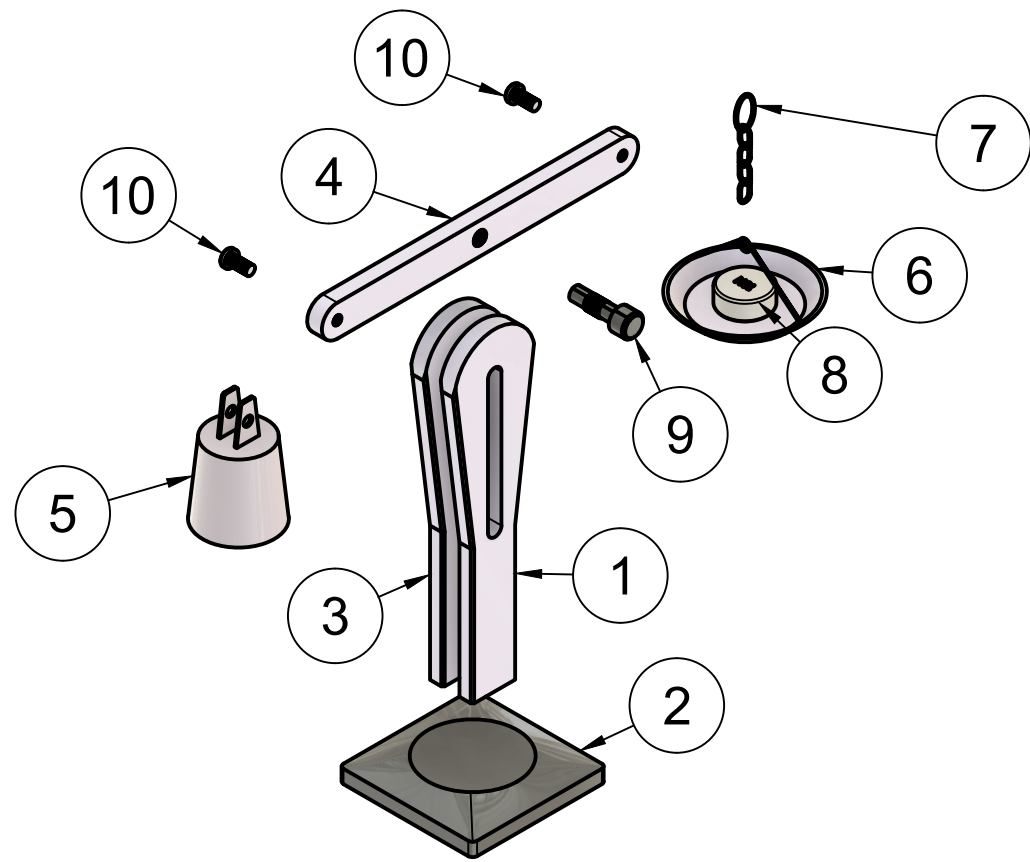
EXPLODED VIEW
