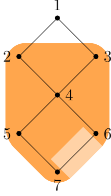
Figure 4: Subgraph J of G in light orange and N_G^2[V(J)] in darker orange
