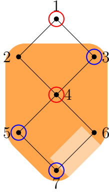
Figure 6: Add S_2 \cap N_G^2[V(J)]
