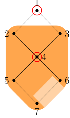
Figure 5: Remove V(J) from S_1
