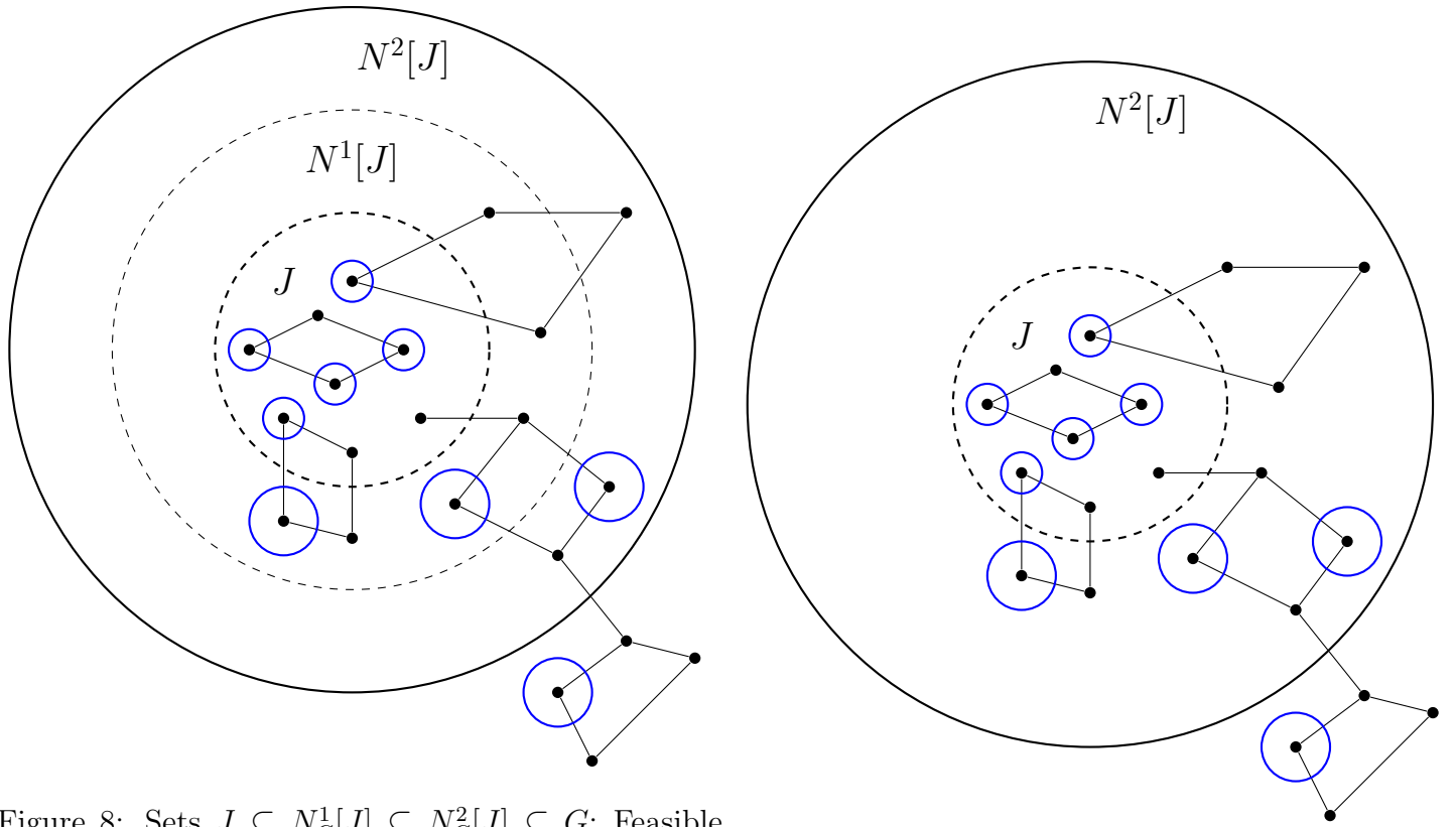
Figure 8: Sets J \subseteq N_G^1[J] \subseteq N_G^2[J] \subseteq G ; Feasible solution S_1 colored in blue.
