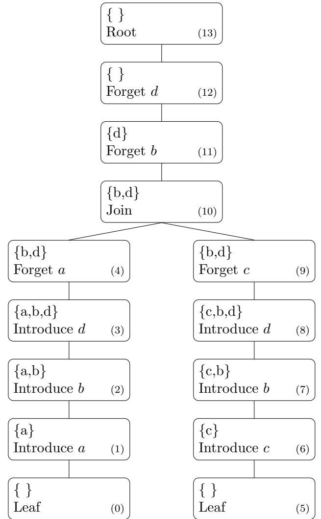
Figure 16: Alternative Tree Decomposition with Join Node at \{b,d\}
