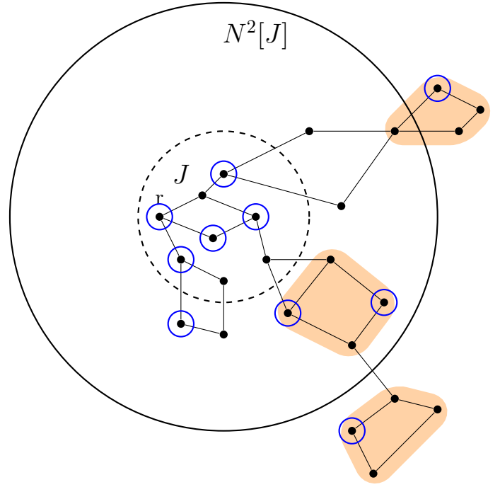
Figure 9: \forall v \in \{v_1, v_2, v_3, v_4\} , such that v_1 v_2 v_3 v_4 is a four cycle: v \notin J
