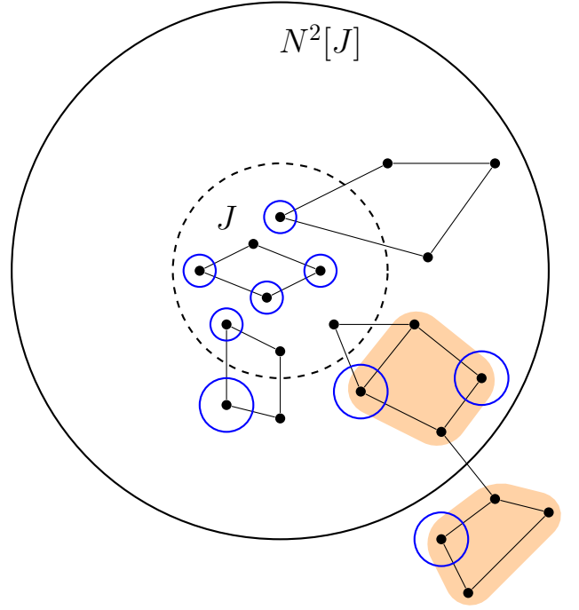
Figure 9: 4-cycles \forall v \{v_1, v_2, v_3, v_4\} : v \notin J
