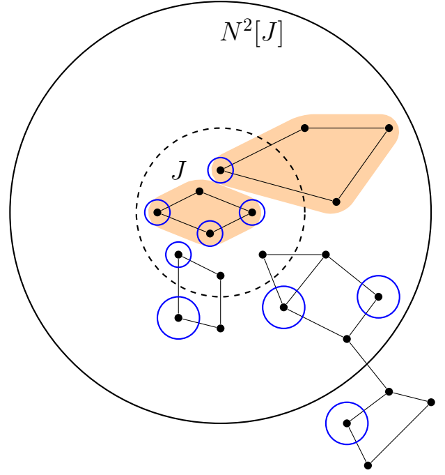
Figure 11: \forall v \in S_1 : v \in J
