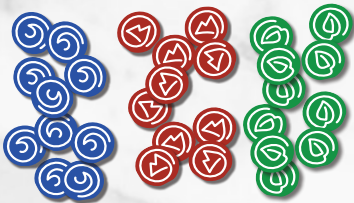
75 ELEMENT TOKENS
