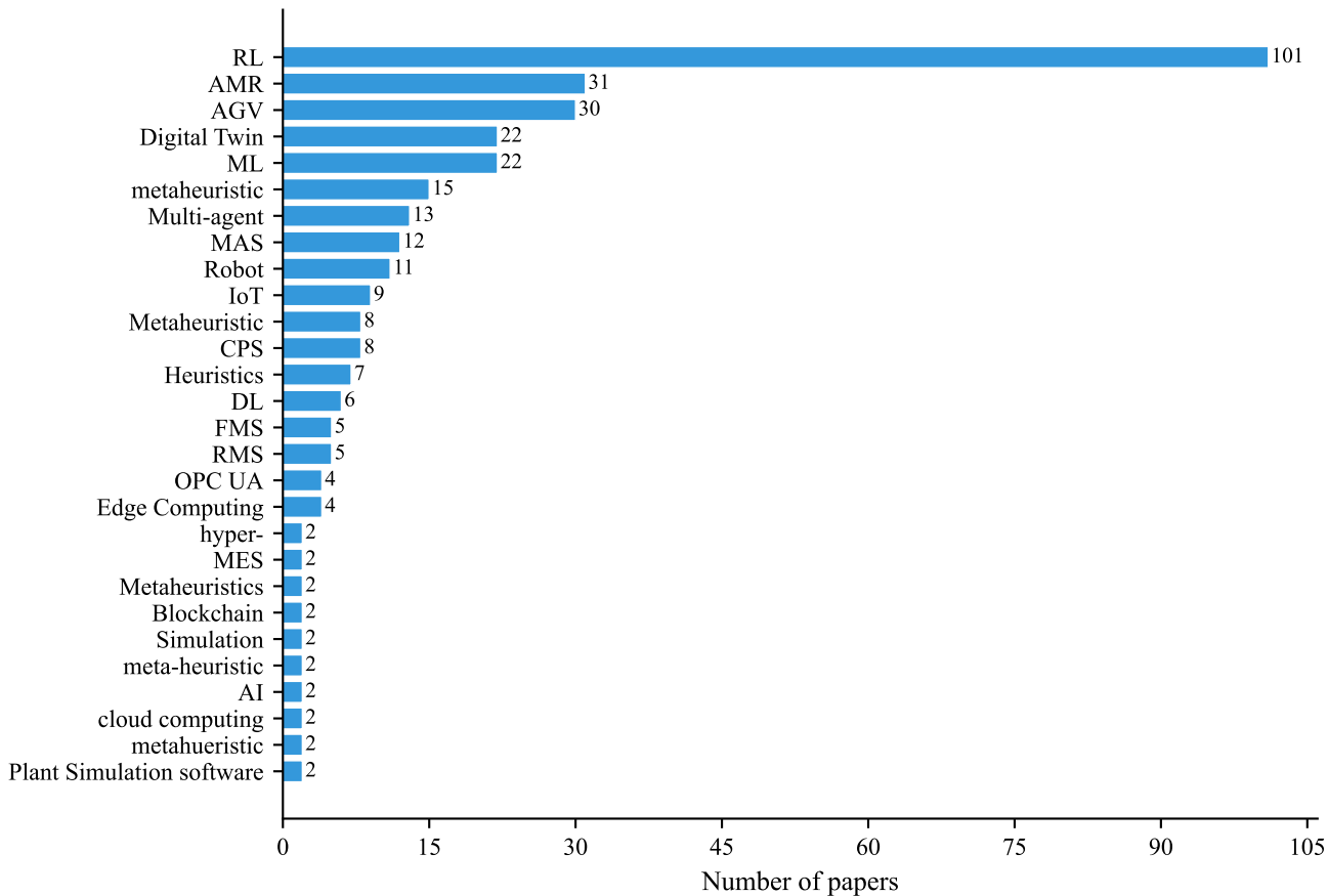
Technology adoption across studies ( \geq 2 occurrences)
