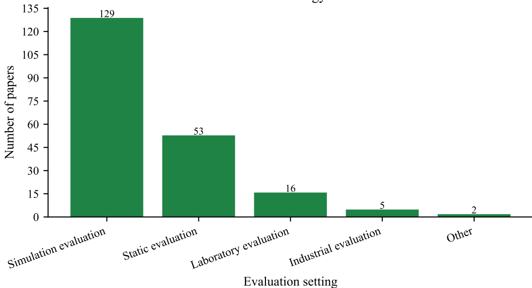
Evaluation methodology distribution
