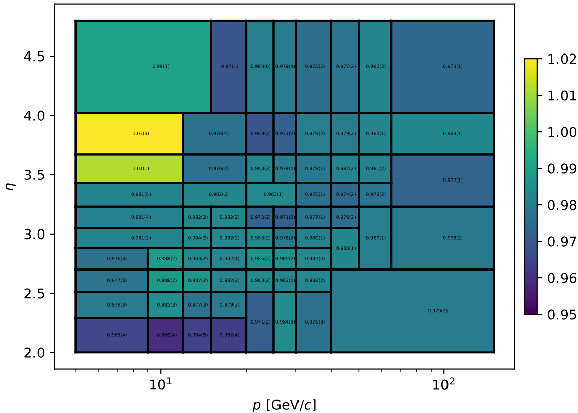
2025 Block 3 Data/MC tracking efficiency ratios
