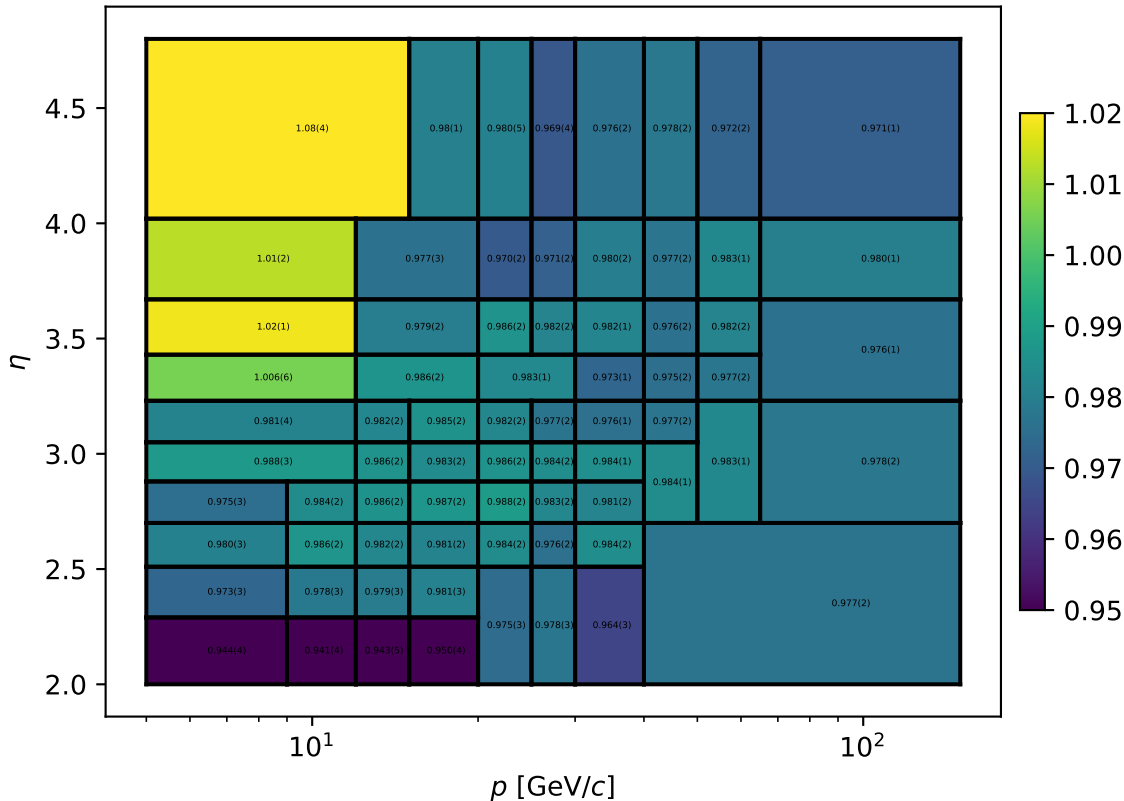
2025 Block 4 Data/MC tracking efficiency ratios
