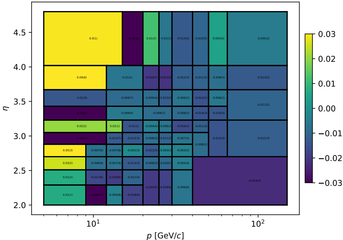
2025 Block 5 Data/MC Combined vs MuonUT ratio difference
