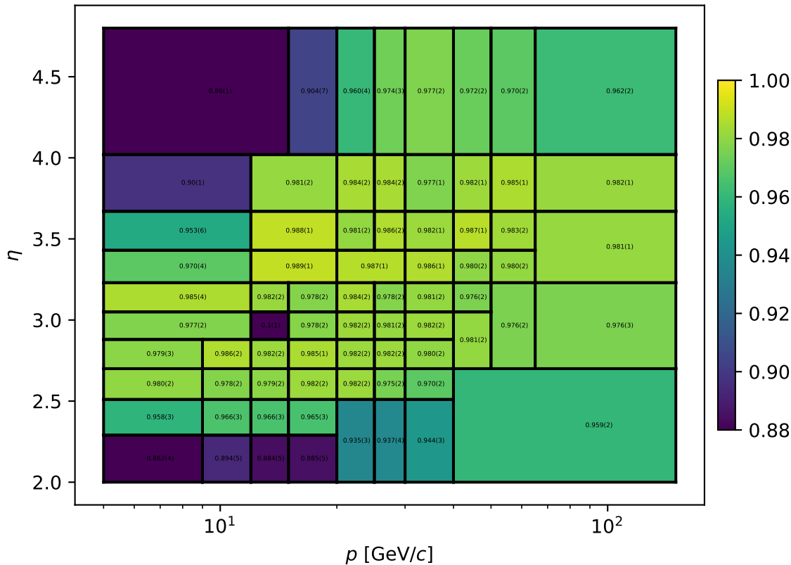
2025 Block 1 MC tracking efficiencies
