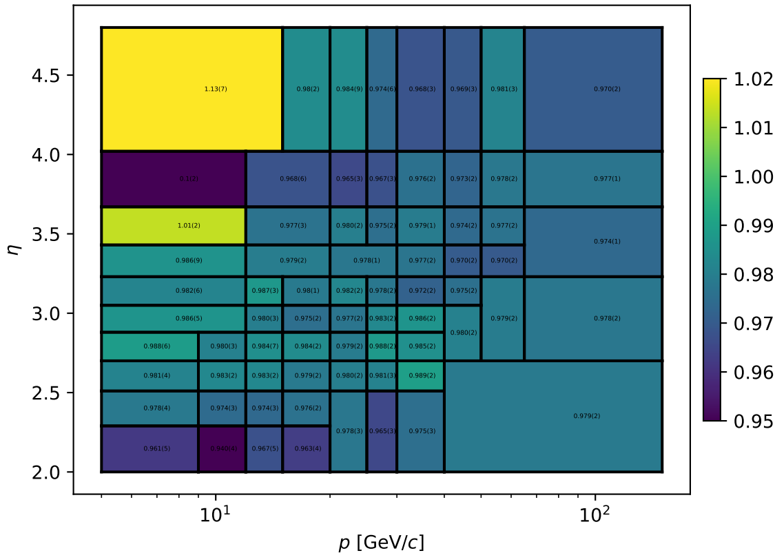
2025 Block 5 Data/MC tracking efficiency ratios
