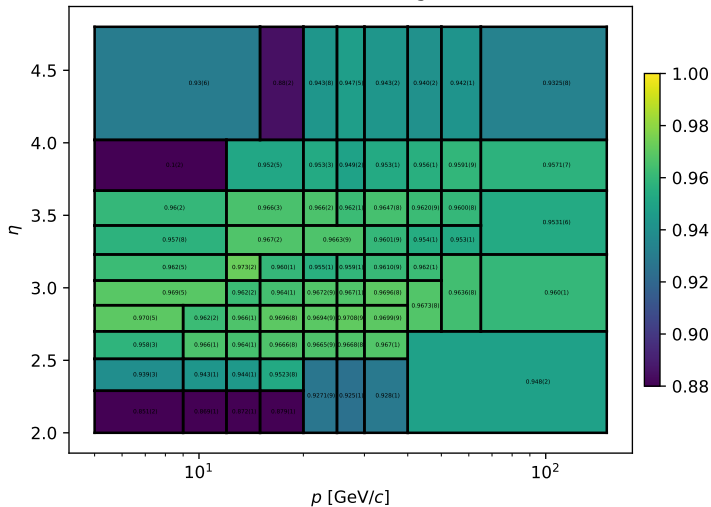
2025 Block 5 Data tracking efficiencies
