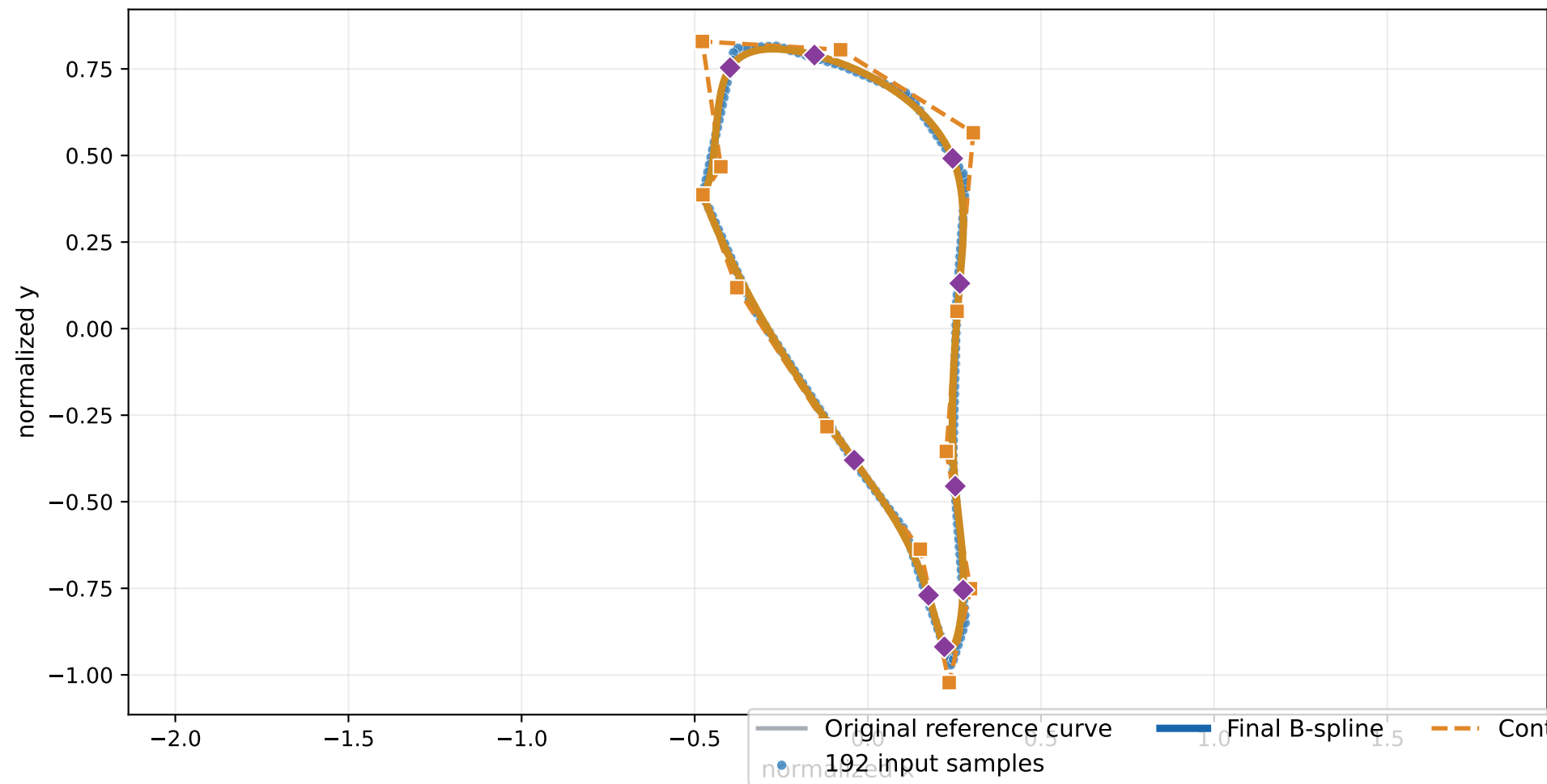
Kang 2015 (ADMM adaptation) — PASS input MSE= 8.36\text{e-}05 | ref MSE= 8.57\text{e-}05 | K=9 full method=304.98 ms
