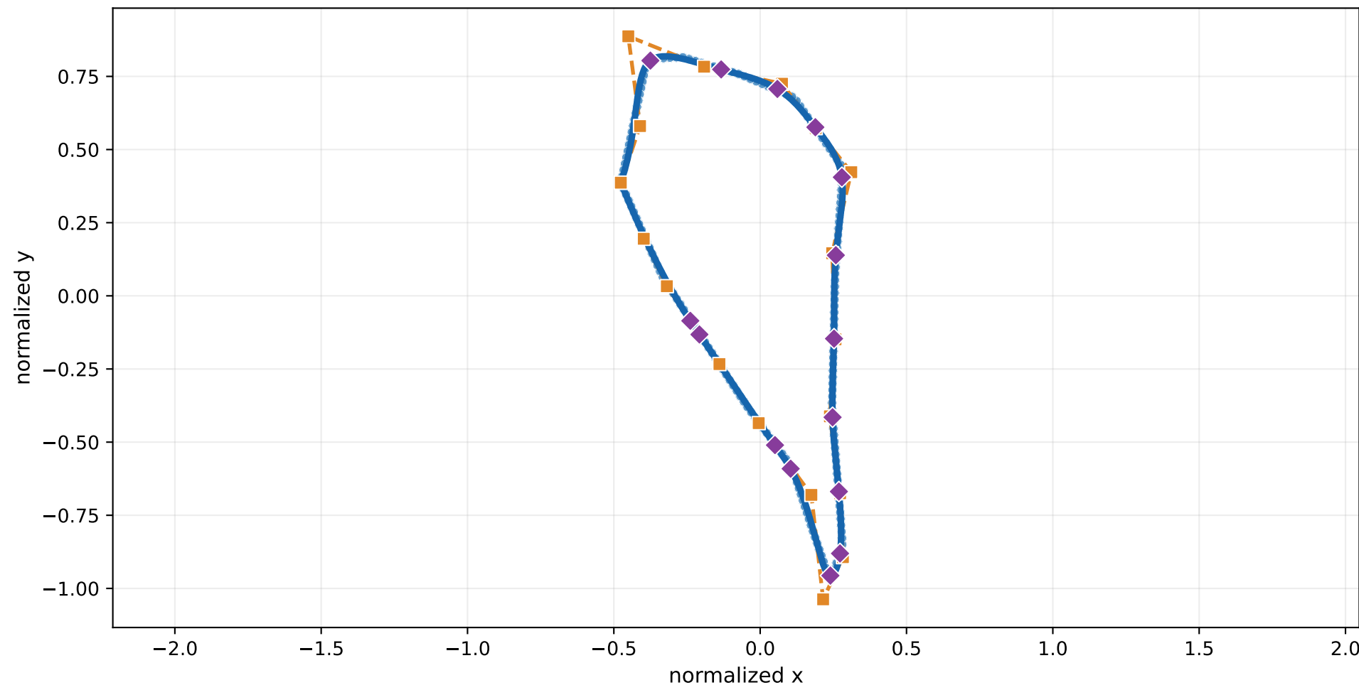
Liang et al. 2017 (feature-IKI adaptation) — PASS input MSE= 9.65\text{e-}05 | ref MSE= 9.81\text{e-}05 | K=10 full method=10.37 ms
