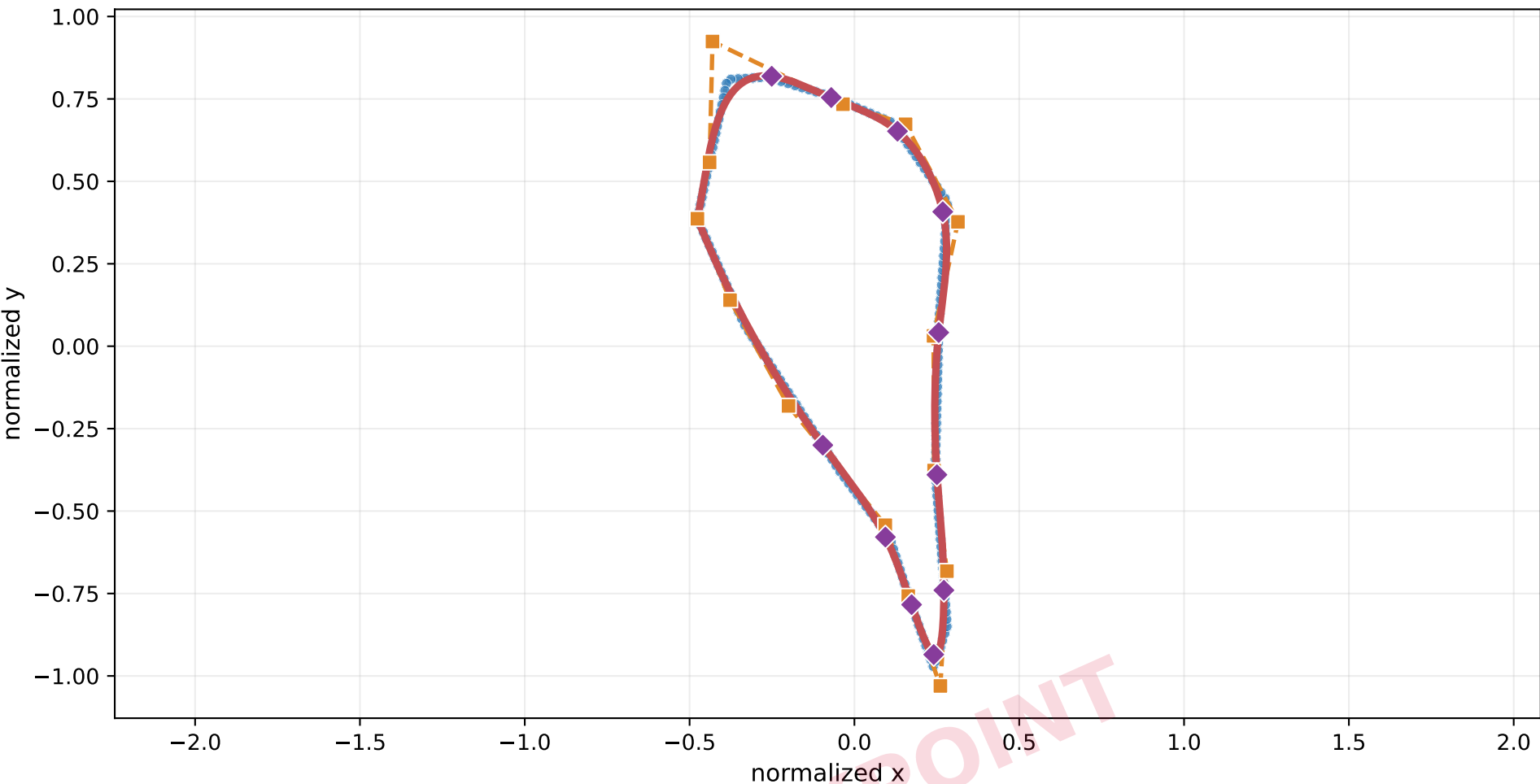
Dung & Tjahjowidodo 2017 (serial adaptation) — FAIL input MSE= 5.56\text{e-}04 | ref MSE= 5.65\text{e-}04 | K=6 full method=90.84 ms
