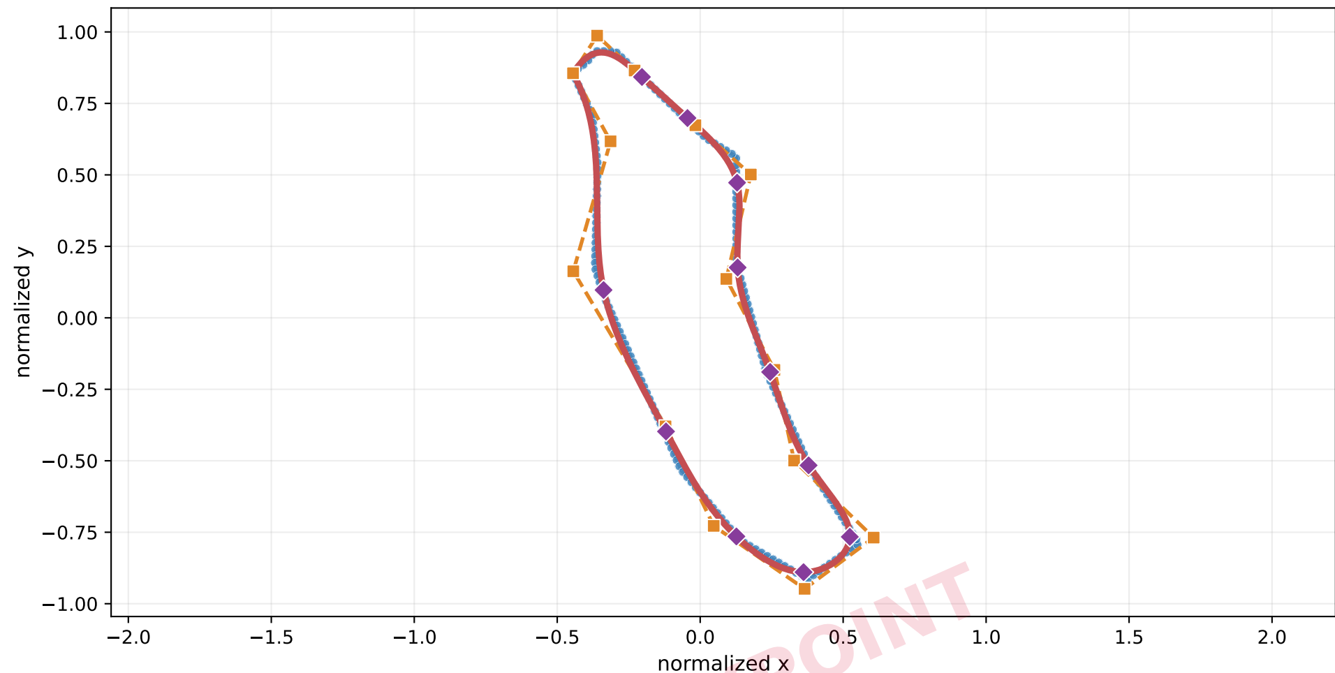
Dung & Tjahjowidodo 2017 (serial adaptation) — FAIL input MSE=3.14e-03 | ref MSE=3.17e-03 | K=5 full method=78.21 ms
