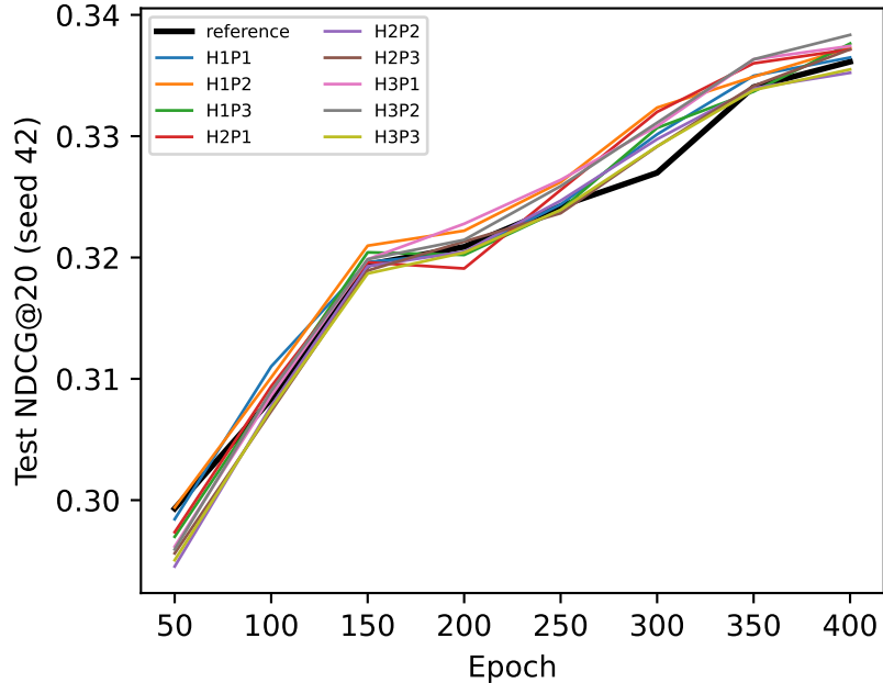
Training curves (not used for selection)
