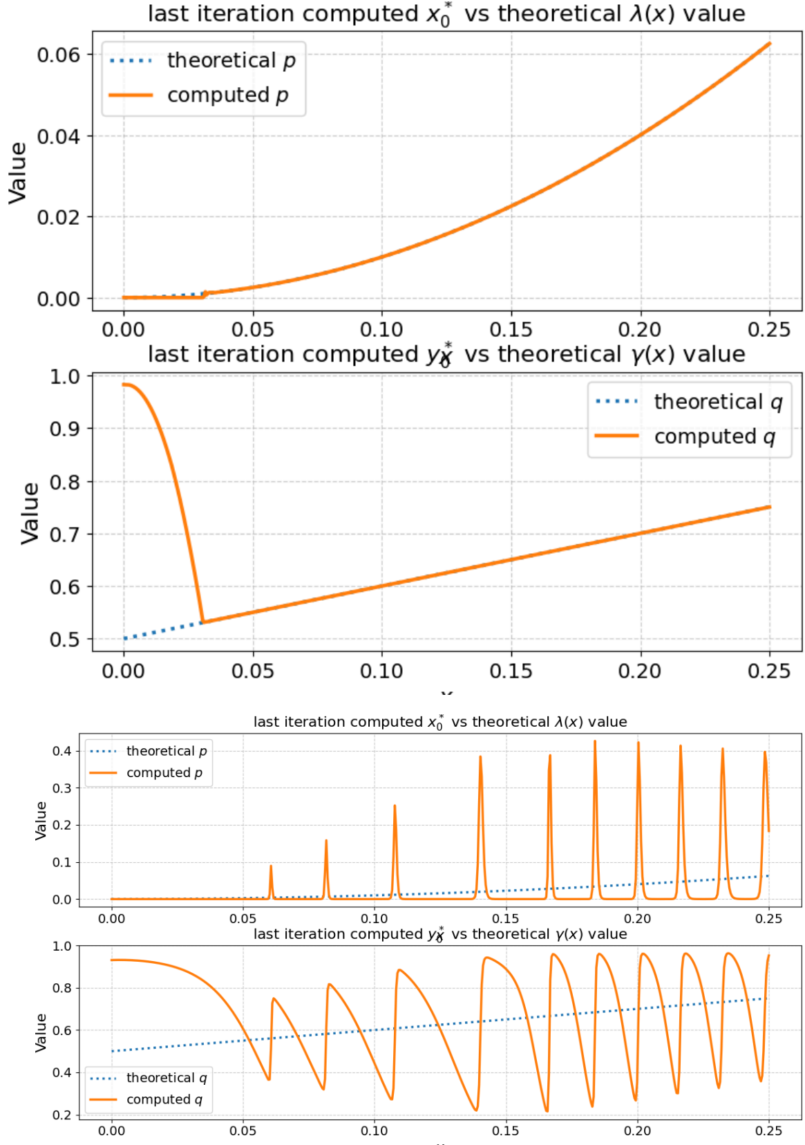
Figure 4: Evolution of computed last-iterate strategies against theoretical Nash Equilibrium probabilities for OGDA (left) and OMWU (right).
