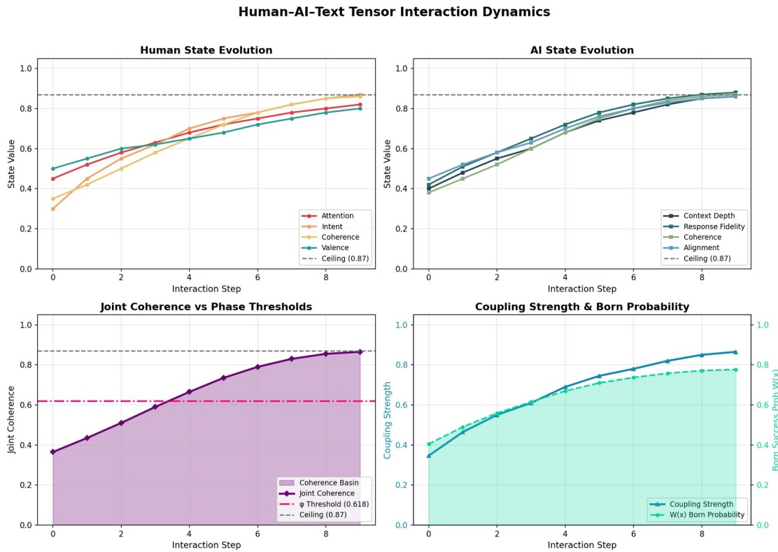
Figure 5.1: Tensor Lab v0.2 reference session (tensor_run_01_v2_corrected.csv) showing the textbook gradual-tear trajectory: H/AI state evolution into the 0.87 ceiling, joint coherence rising past the 0.618 threshold, with coupling strength and Born-rule success probability rising in lockstep.
