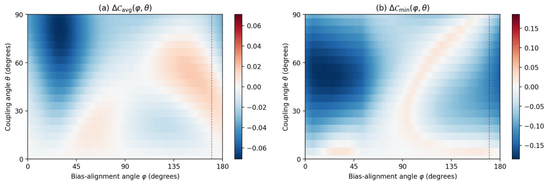
Paper 9, Fig. 1: Conditional improvement region for the seeded G_2 -structured affine dyad (a) averaging functional: 24.6% of cells gain; (b) minimum functional: 12.5% of cells gain. r_A = r_B = 0.7 ; R_A, R_B random orthogonal in 14D (seeds 20260504/20260505).
