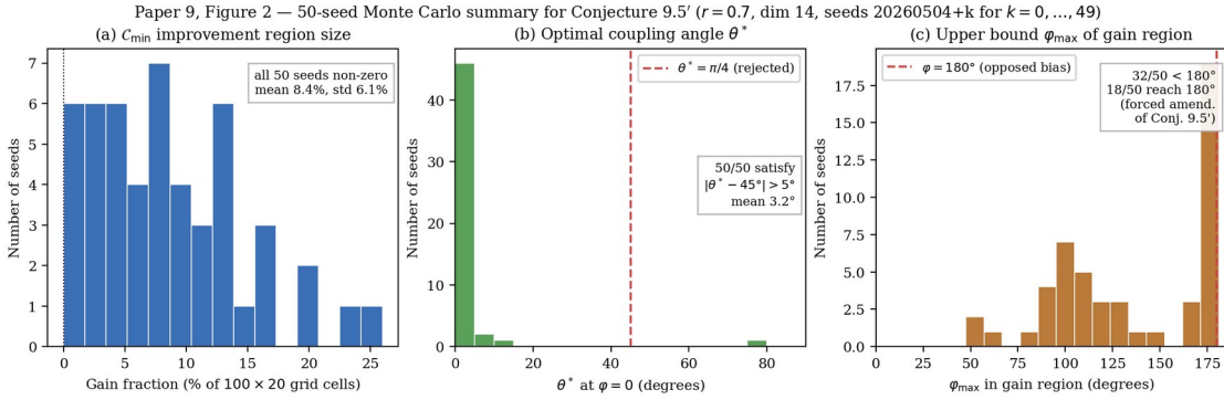
Paper 9, Fig. 2: 50-seed Monte Carlo summary for Conjecture 9.5'. Each panel shows a histogram across the 50 seeded (R_A, R_B) pairs (seeds 20260504+k for k=0, \dots, 49 , r=0.7 , dim 14). (a) Gain-region size, expressed as the percentage of 100 \times 20 grid cells in (\varphi, \theta) -space where \Delta C_{min} > 10^{-10} ; all 50 seeds are non-zero, with mean 8.4 % and standard deviation 6.1 %. (b) Optimal coupling angle \theta^i at aligned bias ( \varphi=0 ); all 50 seeds satisfy |\theta^i - 45^\circ| > 5^\circ , with the dashed red line marking the rejected universal \pi/4 value. Most seeds favor very small \theta^i (mean 3.2^\circ ). (c) Upper bound \varphi_{max} of the improvement region; 32/50 seeds are bounded below the dashed red opposed-bias line at \varphi = 180^\circ , while 18/50 admit small- \theta improvement cells extending up to 180^\circ —this latter behavior forced the amendment of Conjecture 9.5' to drop the original “bounded strictly away from opposed biases” clause. Reproducible from computations/paper9_conjecture95_mc_seeds.csv via figures/build_fig2_mc.py .
