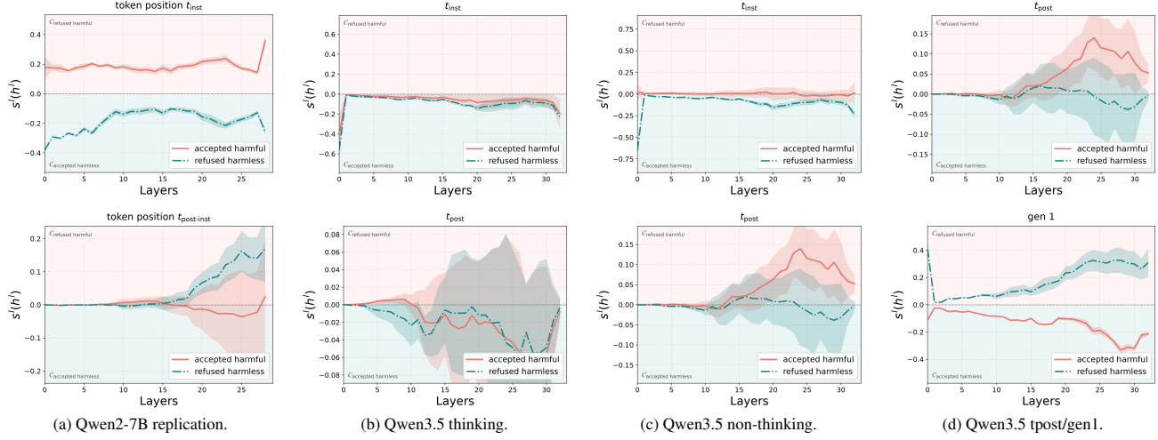
Figure 3: Layer-wise activation score curves for selected token positions. The Qwen2-7B panel reproduces the original prompt-boundary pattern, while the Qwen3.5 panels compare thinking and non-thinking token choices.
