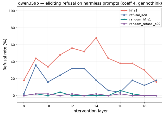
Figure 5: The orange and blue curves show the refusal rates under additive steering in the harmfulness direction (orange curve) and refusal direction (blue curve). In addition, we randomly rotated the steering vectors v_l^{\text{harmful}} and v_l^{\text{refuse}} to produce two random steering directions. The results of random steering are given by the green and purple curves. The steering coefficient is set to c = 4 in all cases, and the thinking mode is disabled.
