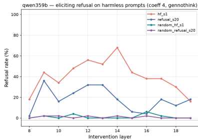
Figure 5: Layer-wise refusal elicitation after steering along the estimated harmfulness and refusal directions.
