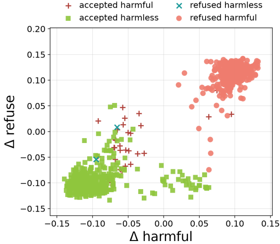
Figure 7: Harmfulness/refusal scatter for Qwen3.5-9B in the thinking setting. The two axes separate input harmfulness from refusal behavior, supporting the claim that the concepts are represented separately rather than as one monolithic safety signal.
