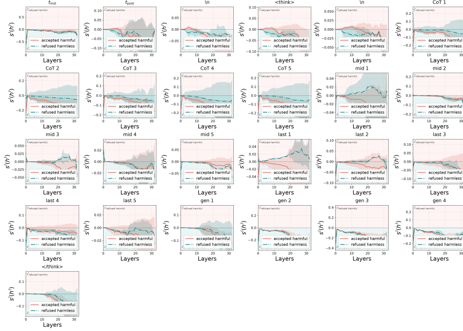
Figure 6: Score curves for Qwen3.5-9B in the thinking setting. The multi-slot layout extends the original t_{\text{inst}}/t_{\text{post-inst}} analysis to prompt, think-template, CoT, \langle \text{think} \rangle , and answer positions.
