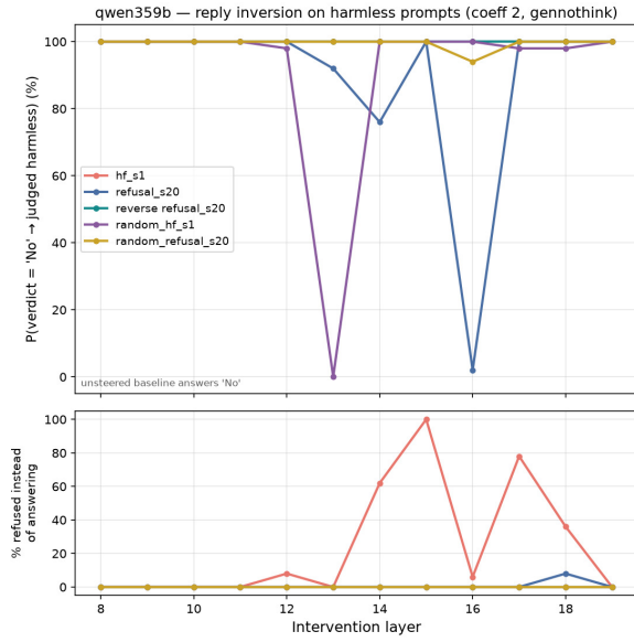
(a) Unsteered model answers “No” at 100% rate. Adding v_l^{\text{harmful}} makes the model not answering at all.
