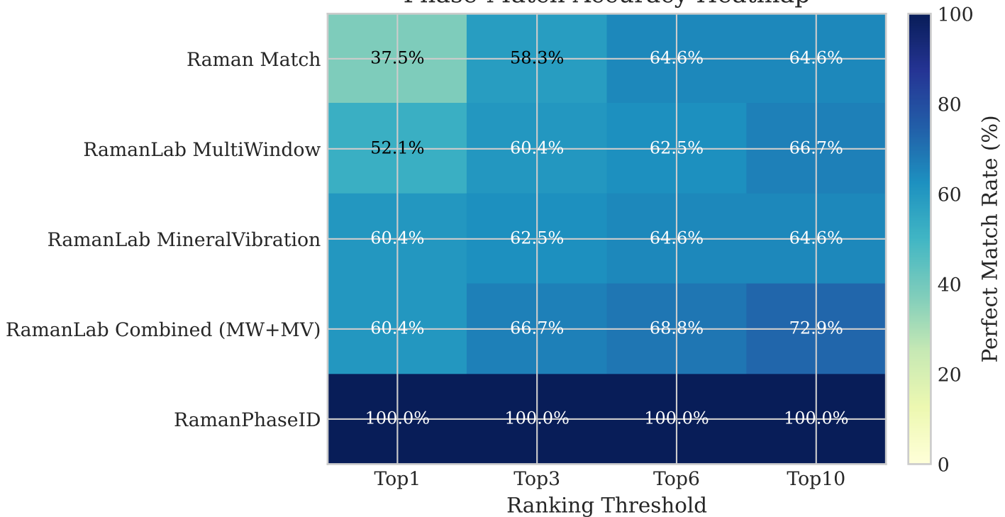
Phase-Match Accuracy Heatmap
